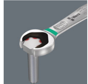
Integrated limit-stop
